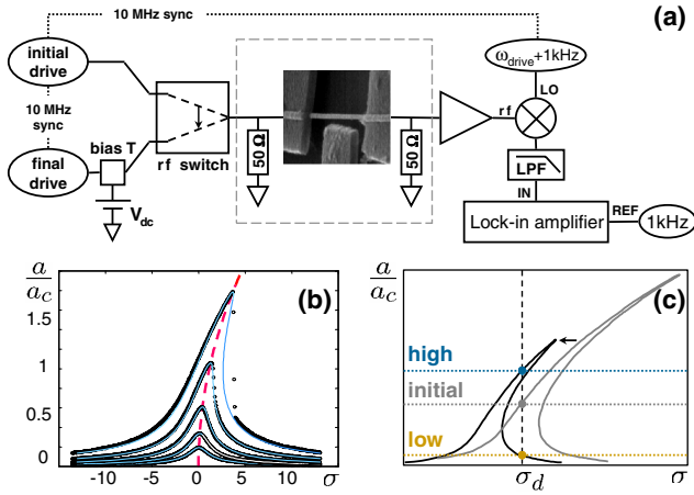
FIG. 1 (color online). (a) Experimental layout. The initial drive prepares an initial state of the platinum nanowire resonator (shown in the SEM photo), a 5 ns rf switch is then flipped to connect to the final drive, and the state of the device is measured by a lock-in amplifier after mixing down to a low (1 kHz) frequency and low-pass filtering (LPF) the residual rf signal. (b) Vibration amplitude versus frequency, for various driving powers at the sample ( -90 , -85 , -80 , -75 , -70 dBm, or normalized to the critical drive V_c = 28.4 \mu\text{V} , V/V_c = 0.249 , 0.443 , 0.788 , 1.401 , 2.492 ) showing the onset of nonlinearity in the platinum nanowire resonator. (c) The state of the nanowire resonator is first prepared in an initial state on the initial response curve (gray) by choosing an appropriate drive strength for the fixed detuning frequency, \sigma_d = 4.26 . After the rf switch is flipped to connect the final drive, the response curve changes to the one shown in black and the initial state evolves to either the high-amplitude state or low-amplitude state. The small bias voltage, applied to the nanowire together with the final drive, is chosen so that the hysteresis loop of the initial curve is at higher frequency than the operating frequency.
