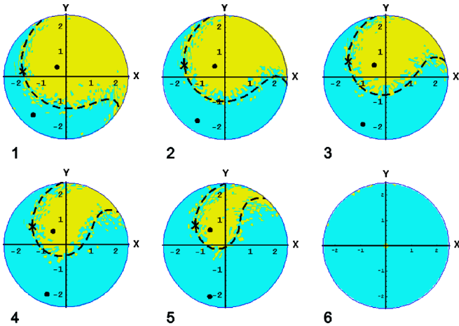
FIG. 2 (color online). Basins of attraction of a nanowire resonator at a fixed frequency, \sigma_d = 4.26 , for increasing final drive values, V_f/V_c = (1)1.867 , (2)2.049, (3)2.237, (4)2.434, (5)2.640, (6)2.741. Blue and yellow colors indicate the final high- and low-amplitude states, respectively. The data consist of 60 concentric circles with 60 points each, corresponding to a displacement range of 0 to 2.5a_c . Theoretical fixed points, saddle point, and separatrix curve are indicated by black points, black cross, and the dashed black curve, respectively.
