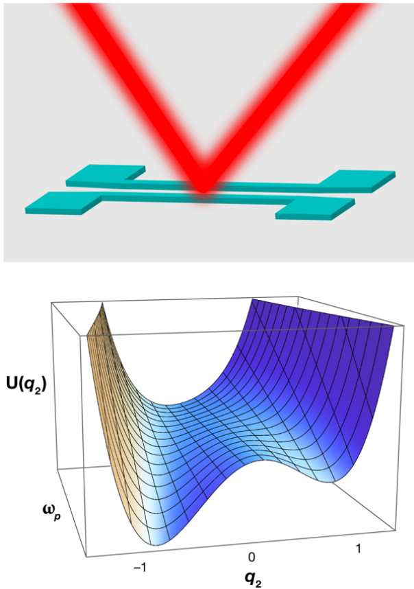
FIG. 1: (Top) A sketch of the system, which is a pair of 6 \times 0.5 \times 0.2 \mu\text{m} doubly clamped nanobeams with 400 nm separation. The beams were illuminated by an infrared laser focused to a spot of 10 \mu\text{m} and the reflected signal was detected. (Bottom) The effective potential for the slow coordinate q_2 of the higher-frequency nanobeam for different values of the modulation frequency \omega_p ; |q_2| gives the scaled amplitude of the vibrations at frequency \omega_p/2 , whereas the sign of q_2 determines their phase. (Credit: Alan Stonebraker)
